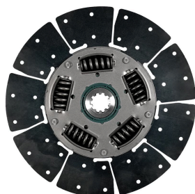
IVECO DAILY 280MM
